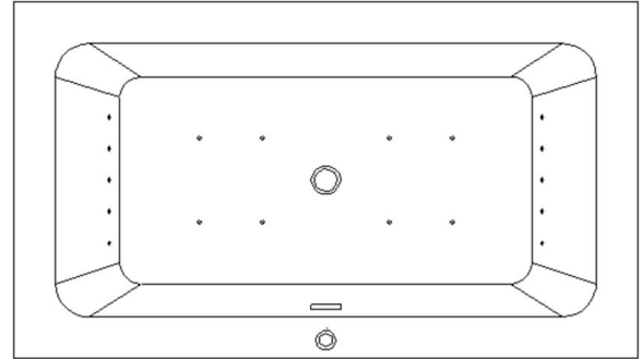
Asti59CAJ (Air Jet) (Electrical: 1x 110V 15A GFCI) Standard Feature: Air Blower
