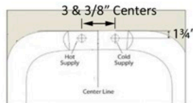
Measurements to be used for rough in plumbing only
